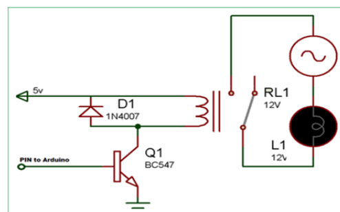
Fig 2: Relay
