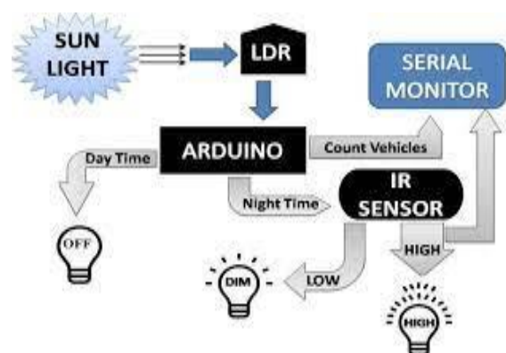
Fig. 2: Street light proposed method
