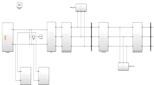
Fig 4.1 MATLAB/SIMULINK circuit of the Grid Connected PV Array and Battery
