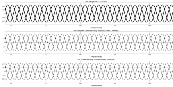
Fig. 4.8 Comparative of the proposed control with fractionalordercorrentropy adaptive filtering algorithm at dc offset
