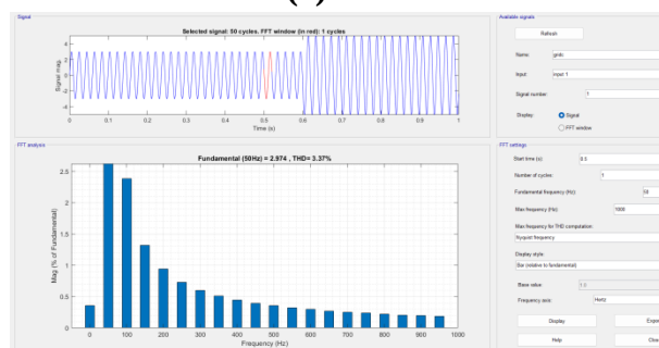
Fig 4.5 THD of grid voltage and grid current
