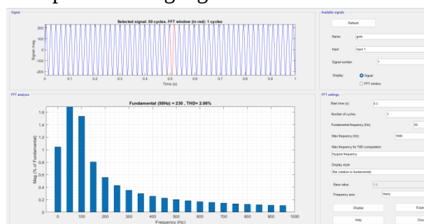
Fig. 4.4 Comparative of the proposed control with fractionalordercorrentropy adaptive filtering algorithm at dc offset
