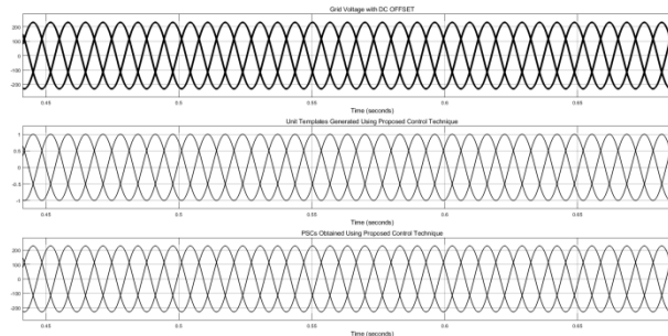
Fig. 4.4 Comparative of the proposed control with fractionalordercorrentropy adaptive filtering algorithm at dc offset
