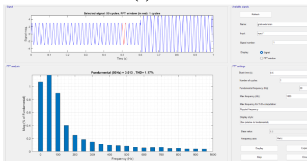
Fig. 4.9 THD of grid voltage and grid current
