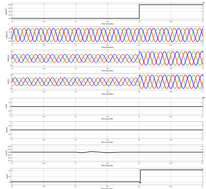
Fig 4.2 Simulated response of EV charging station under variation of PV insolation
