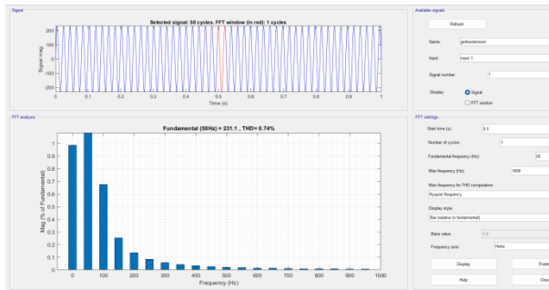
Fig. 4.8 Comparative of the proposed control with fractionalordercorrentropy adaptive filtering algorithm at dc offset
