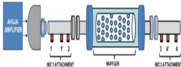
Figure 2 Getting ready for the performance assessments of the mufflers
